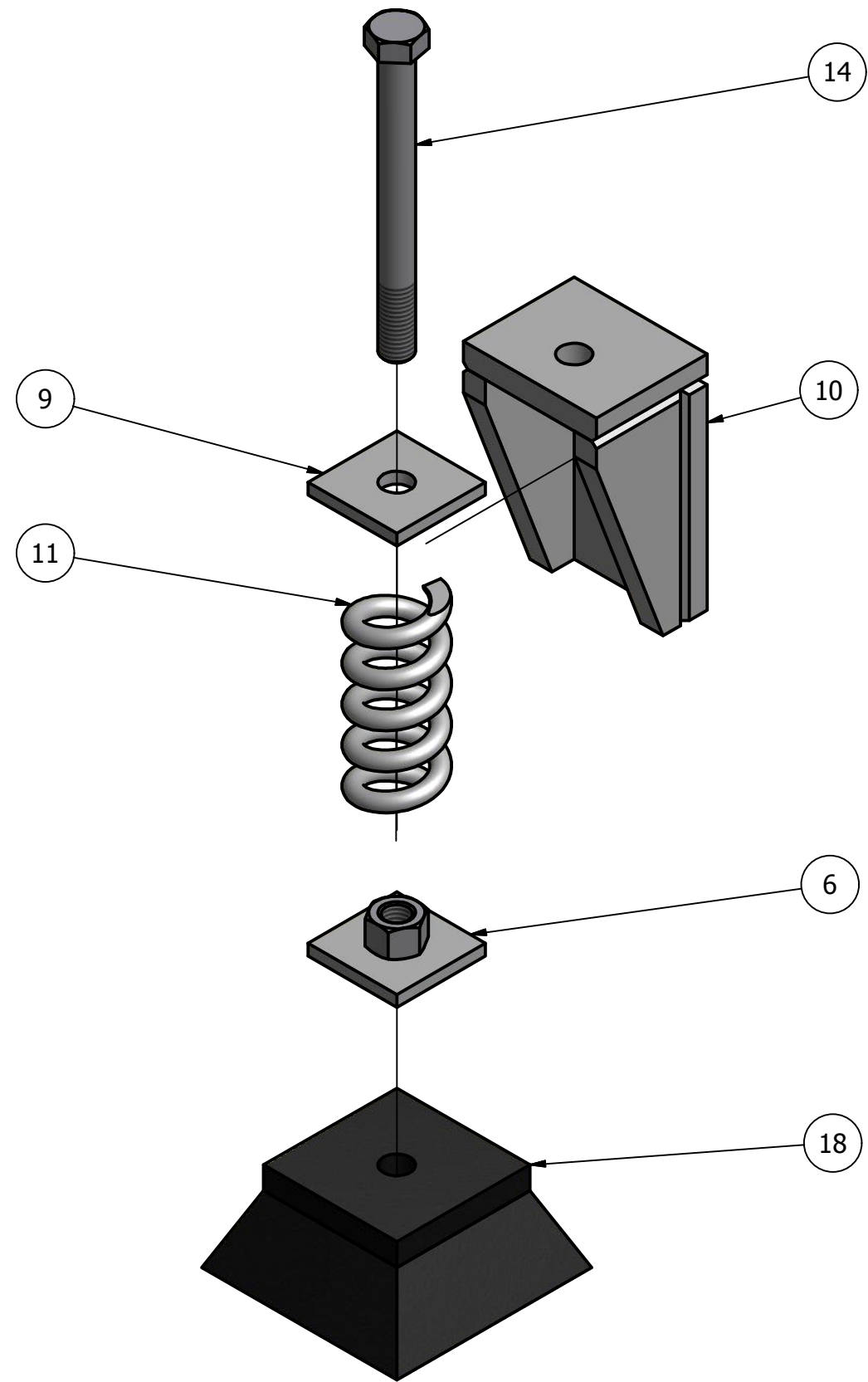
FOOT EXPLODED ASSEMBLY SCALE 1 / 2
