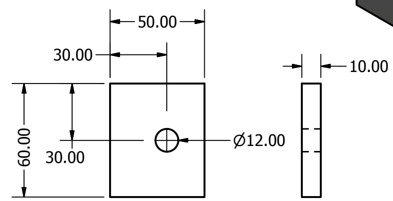
SPRING PLATE BASE SCALE 1 / 2
