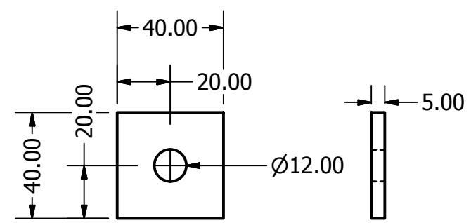
SPRING PLATE SCALE 1 / 2
