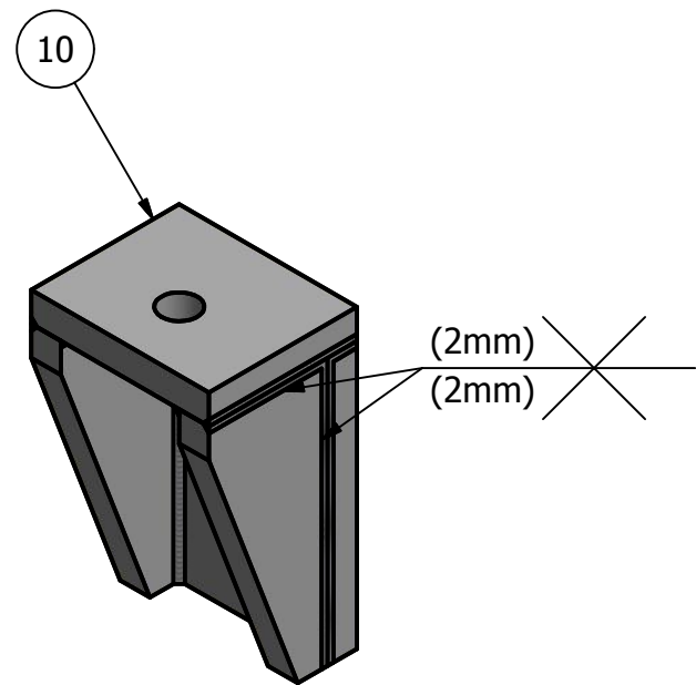
WELDED SPRING PLATE SCALE 1 / 2
