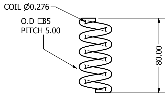
COIL SCALE 1 / 2
