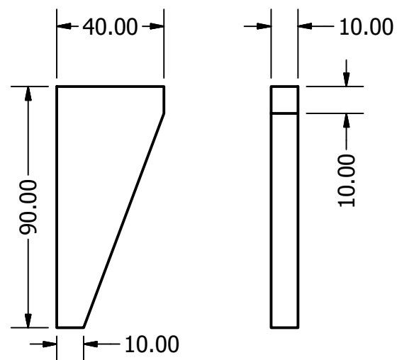
SIDE PLATE SCALE 1 / 2
