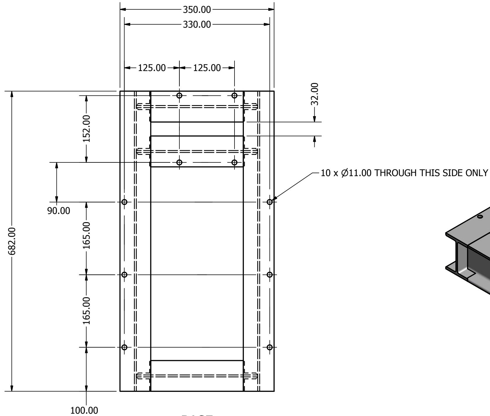
BASE SCALE 1 / 5
