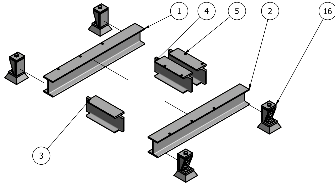
EXPLODED BASE ASSEMBLY SCALE 1 / 10
