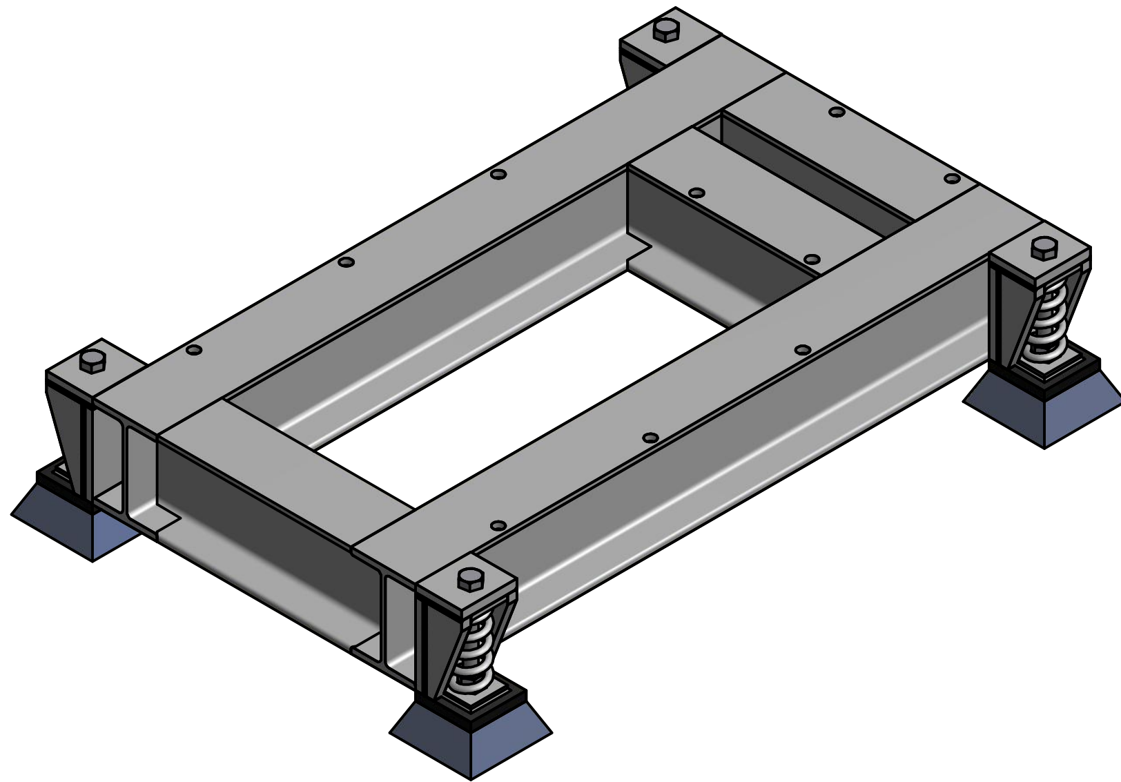
FAN AND MOTOR BASE SCALE 1 / 4
